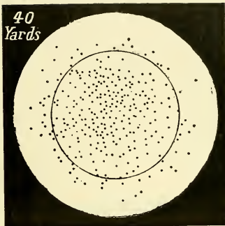
Pattern of CHOKE-BORED Gun at 40 Yards.
